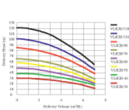
2 x VLR 2 Performance
