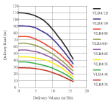
2 x VLR 4 Performance
